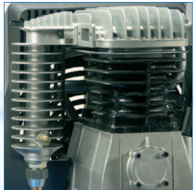
Finned aftercooler for lower temperature compressed air
